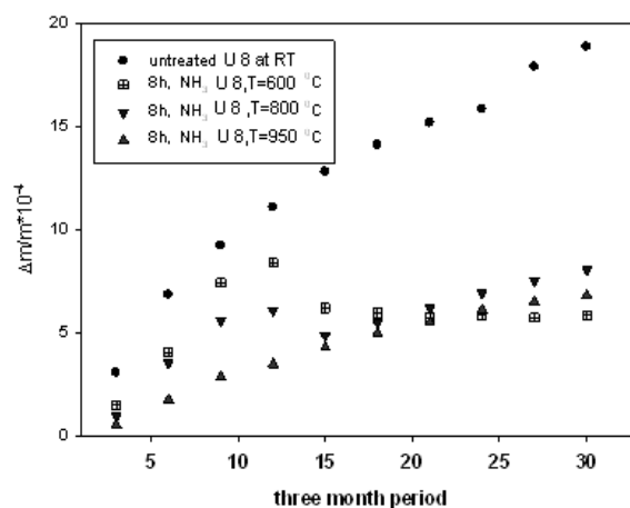
Fig. 5. Resistance of U8 carbon steel after corrosion in seawater for 30 months after NH_3 gas heat treatment
